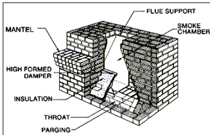
Typical Smoke Chamber Assembly
